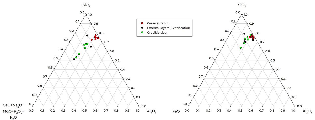
Figure 6. Ternary diagrams comparing the compositions of the ceramic fabrics, external vitrification layers and crucible slag.
