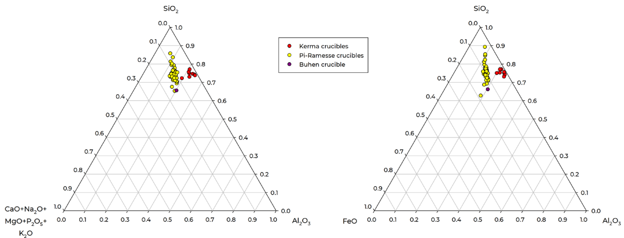
Figure 9. Comparison of ceramic fabric composition between metallurgical crucibles from Kerma (this study), Middle Kingdom Buhen (Davey et al. 2021) and New Kingdom Pi-Ramesse (Rademakers et al. 2018a).
