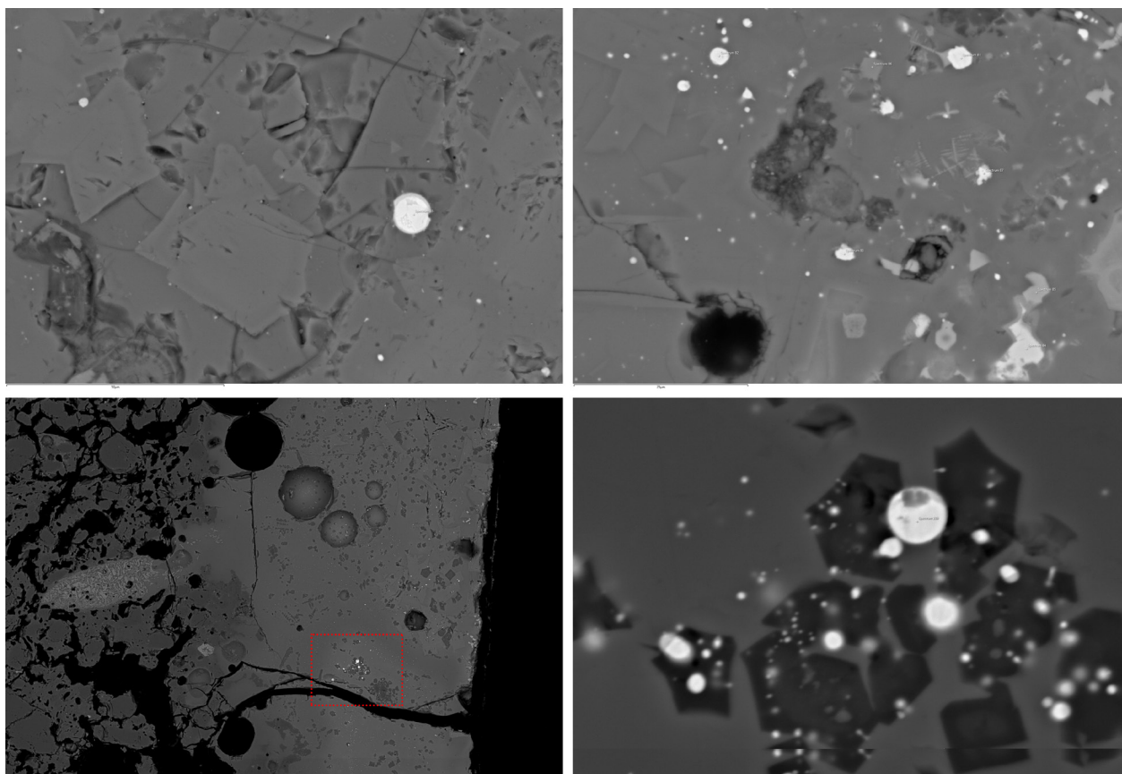
Figure 8. Top left: crucible slag layer in KV1013 including prill with c. 41 wt% arsenic and 31 wt% iron (width of image c. 130µm). Top right, crucible slag layer in KV1013 including prills with c. 20-24 wt% arsenic, 1-4 wt% iron and 2-3 wt% tin (width of image c. 80µm). Bottom left: crucible slag layer in KV 1015 and its transition from the ceramic fabric on the left (width of image c. 0.85mm). Bottom right: close-up of bottom left image showing small copper prills with c. 21 wt% arsenic and 2 wt% iron (width of image c. 0.05mm).
