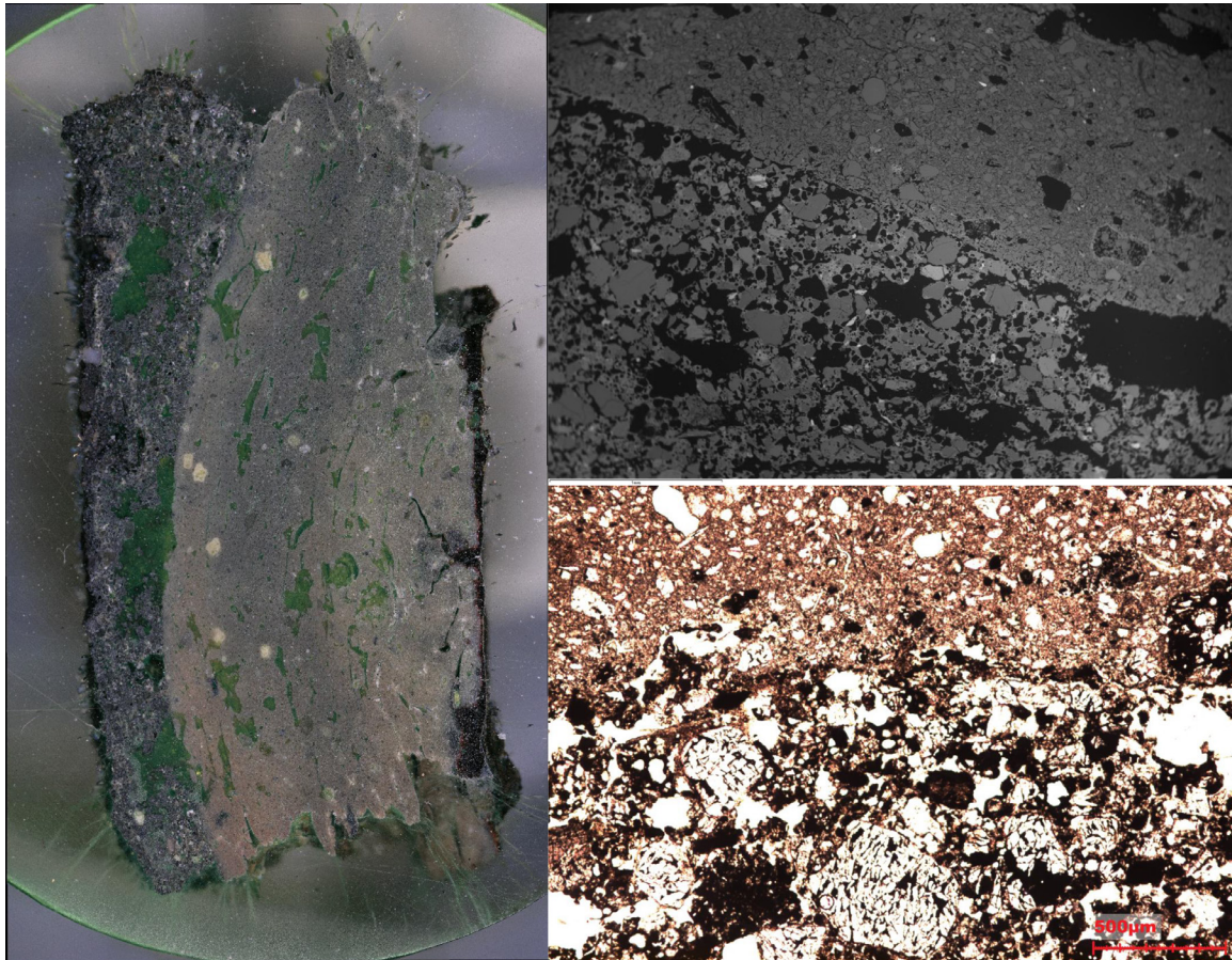
Figure 11. Mounted cross-section of KV 1015 (left) with abrupt transition between externally applied layer, shown in SEM-BSE image (top right, width of image c. 4mm) and PPL micrograph (bottom right, width of image c. 2.5mm).
