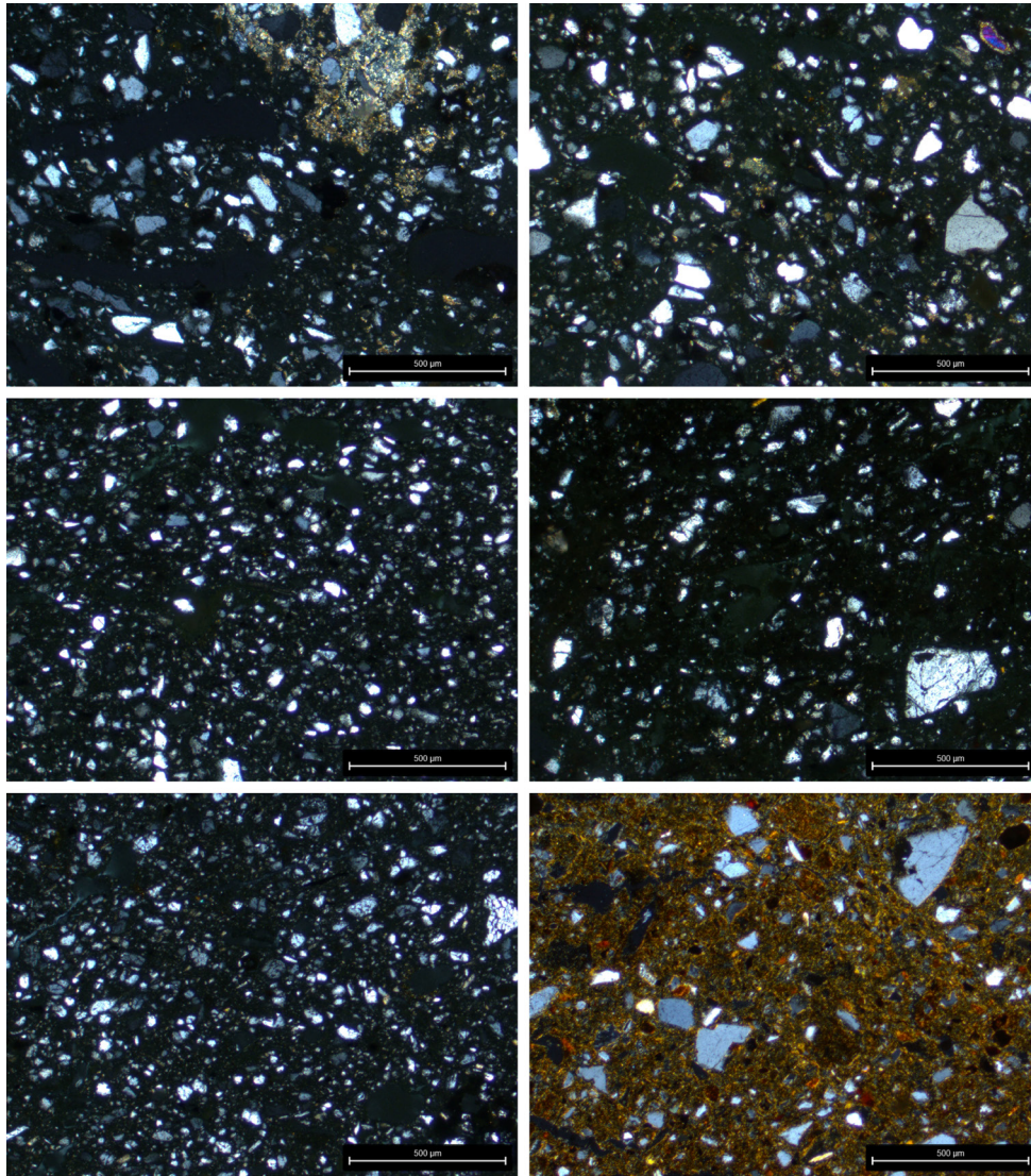
Figure 5. Overview of (core) ceramic fabric of the crucibles in cross-polarised light (XPL). Left to right, top to bottom: KV 1011 and KV 1014, KV 422 and KV 706, KV 1015 and KV 1016.
