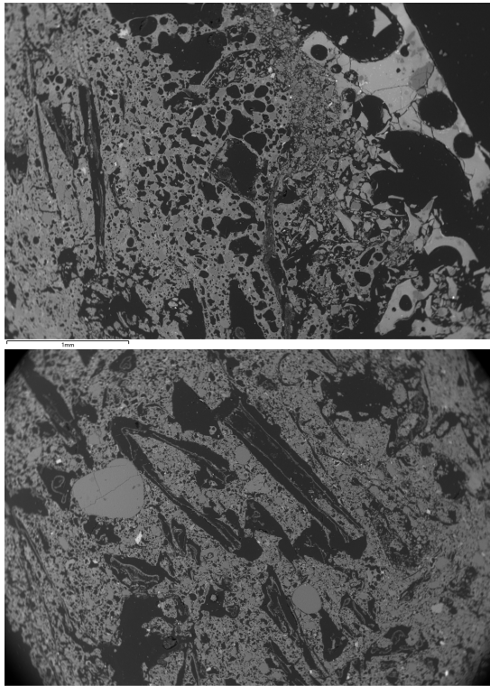
Figure 10. SEM-BSE images of KV 706 (width of images c. 4mm). Top: crucible slag formation at interior, with underlying bloated ceramic. Bottom: porosity from burnt-out organic temper, with residual phytoliths.
