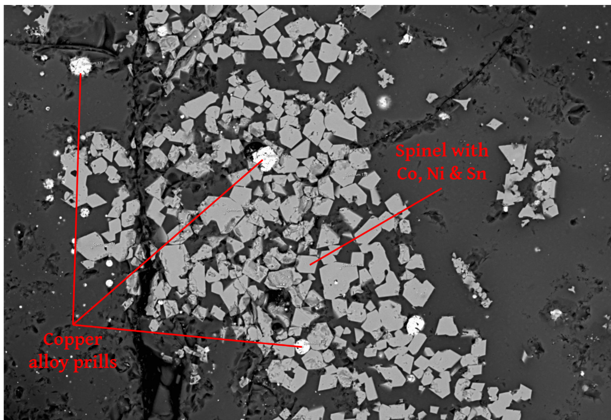
Figure 7. Crucible slag layer in KV 1012 showing arsenical copper prills (2-5 wt% As) with 2.5-5 wt% iron and < 1 wt% nickel, surrounded by spinel (magnetite: \text{Fe}_3\text{O}_4 with c. 1 wt% cobalt, 1.5-2 wt% nickel and up to 0.4 wt% tin) resulting from the (rare) local oxidation of copper alloy prills (width of image c. 0.35mm).
